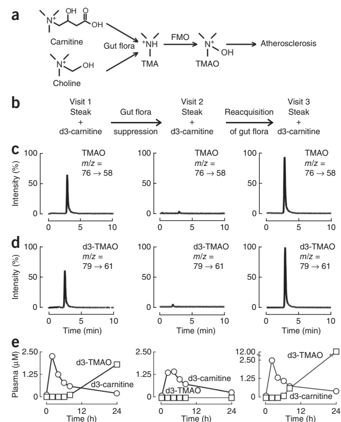
Figure 1 TMAO production from L-carnitine is a microbiota-dependent process in humans. (a) Structure of carnitine and scheme of carnitine and choline metabolism to TMAO. L-Carnitine and choline are both dietary trimethylamines that can be metabolized by microbiota to TMA. TMA is then further oxidized to TMAO by flavin monooxygenases (FMOs). (b) Scheme of the human L-carnitine challenge test. After a 12-h overnight fast, subjects received a capsule of d3-(methyl)-carnitine (250 mg) alone, or in some cases (as in data for the subject shown) also an 8-ounce steak (estimated 180 mg L-carnitine), whereupon serial plasma and 24-h urine samples were obtained for TMA and TMAO analyses (visit 1). After a weeklong regimen of oral broad-spectrum antibiotics to suppress the intestinal microbiota, the challenge was repeated (visit 2), and then again a final third time after a \geq 3 -week period to permit repopulation of intestinal microbiota (visit 3). (c,d) LC-MS/MS chromatograms of plasma TMAO (c) and d3-TMAO (d) in an omnivorous subject using specific precursor \rightarrow product ion transitions indicated at t = 8 h for each visit. (e) Stable-isotope-dilution LC-MS/MS time course measurements of d3-labeled TMAO and carnitine in plasma collected from sequential venous blood draws at the indicated time points. Data shown in c–e are from a representative female omnivorous subject who underwent carnitine challenge. Data are organized vertically to correspond with the visit schedule indicated in b.
